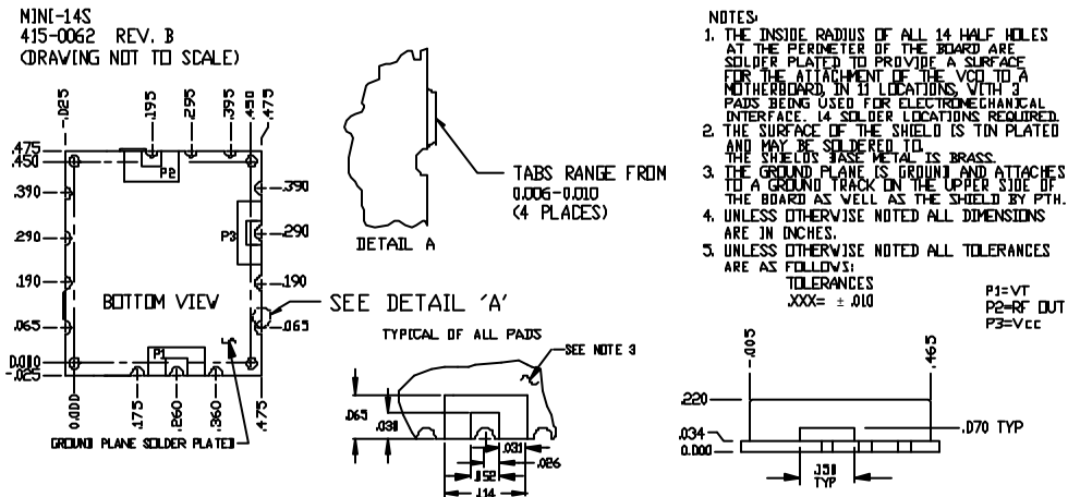
PHYSICAL DIMENSIONS
