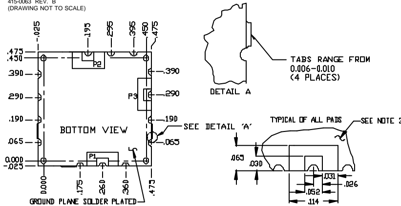
PHYSICAL DIMENSIONS
