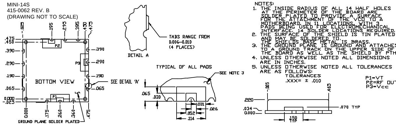
PHYSICAL DIMENSIONS
