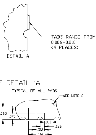
PHYSICAL DIMENSIONS
