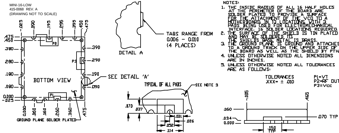
PHYSICAL DIMENSIONS
