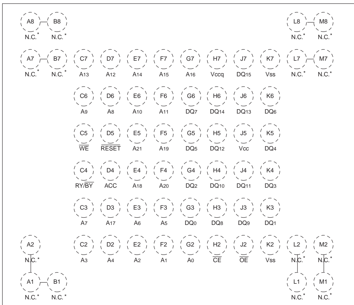
BGA-63P-M02
