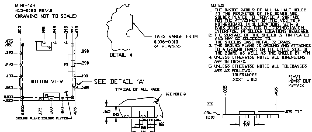
PHYSICAL DIMENSIONS
