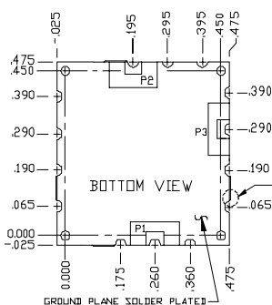
DETAIL A
