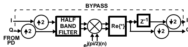
FIGURE 6. IF CONVERTER IN REAL 2X MODE OPERATION
