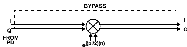
FIGURE 8. IF CONVERTER IN COMPLEX MODE OPERATION
