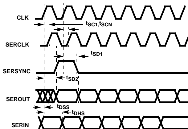
FIGURE 16. SERIAL INTERFACE RELATIVE TIMING
