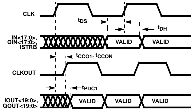
FIGURE 17. INPUT/OUTPUT TIMING
