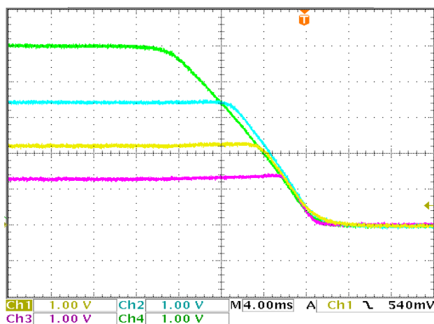
FIGURE 21. OUTPUT VOLTAGE HIGH TO LOW TRACKING
