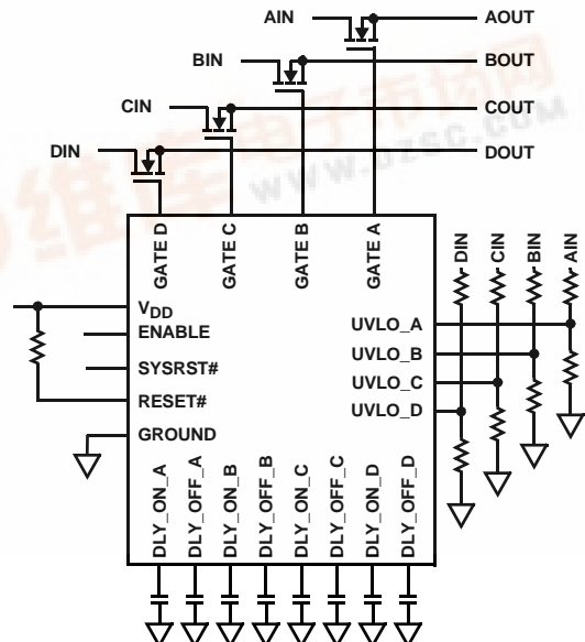
FIGURE 1. TYPICAL ISL6123 APPLICATION USAGE
