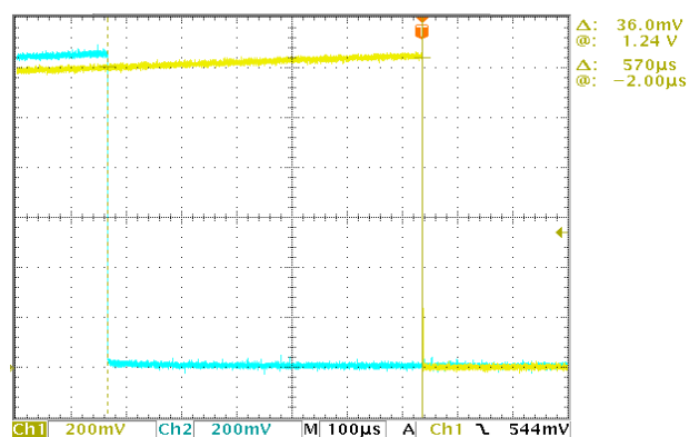
FIGURE 26. CAPACITOR TIMING MISMATCH
