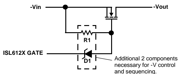
FIGURE 22. ±VOLTAGE SEQUENCING
