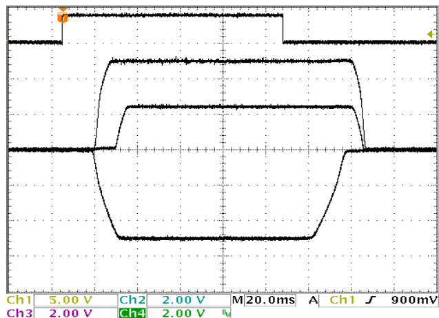
FIGURE 22. ±VOLTAGE SEQUENCING
