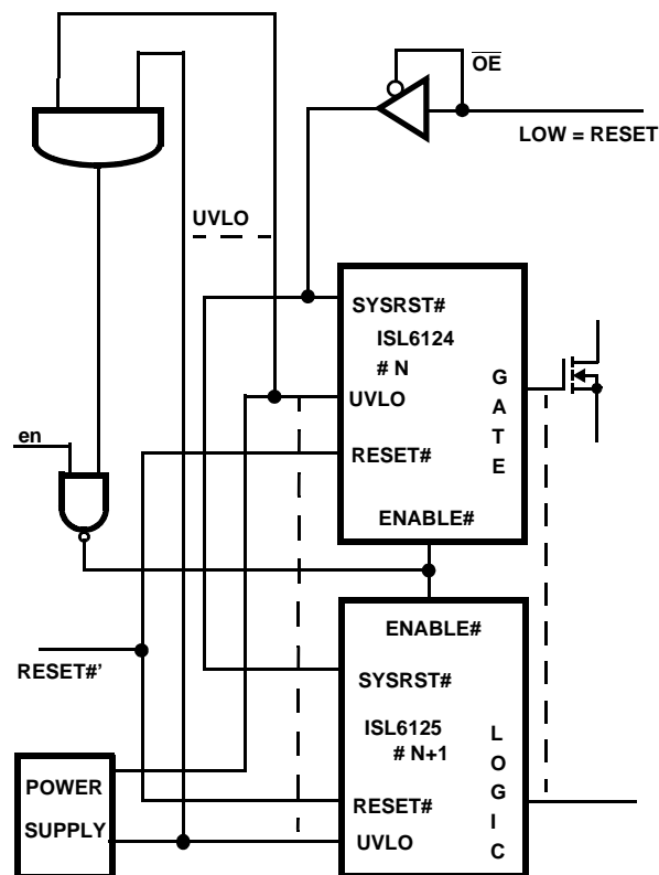
FIGURE 18. MULTIPLE ISL612X USING LOGIC GATES FOR VOLTAGE PRESENCE DETECT
