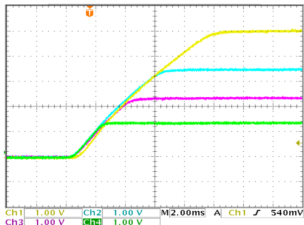
FIGURE 20. OUTPUT VOLTAGE ON LOW TO HIGH TRACKING
