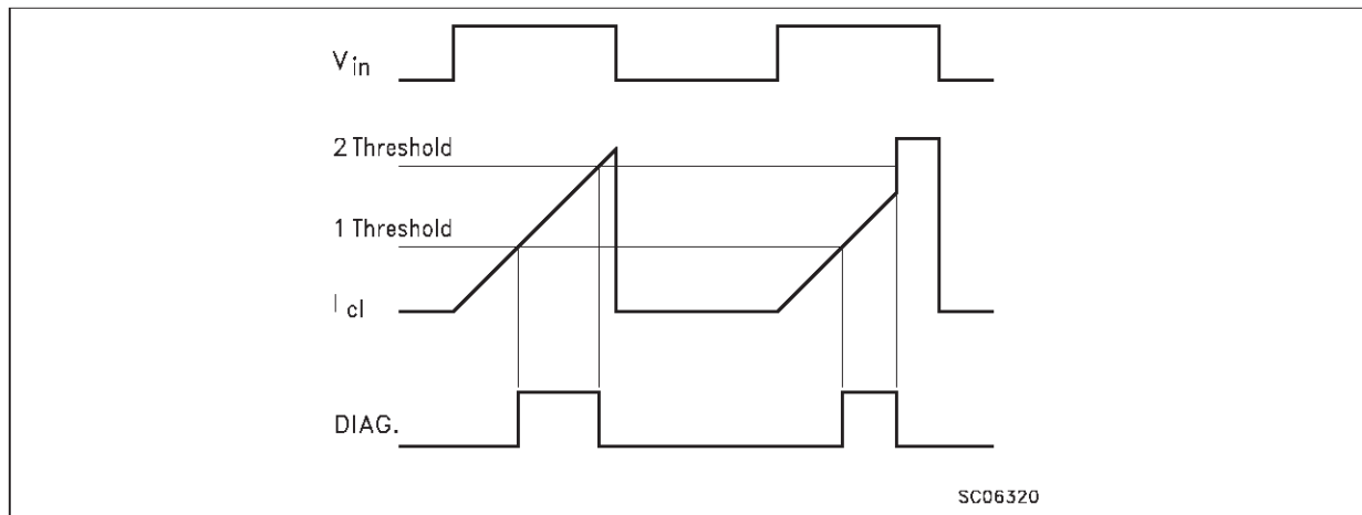
FIGURE 2: Switching Waveforms
