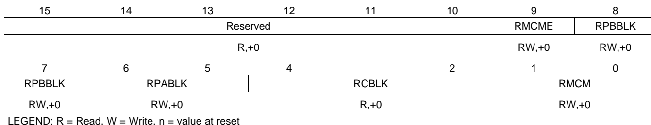
Figure 3-12. Multichannel Control Register 1x (MCR1x)
