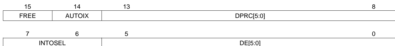
Figure 3-22. DMPREC Register
