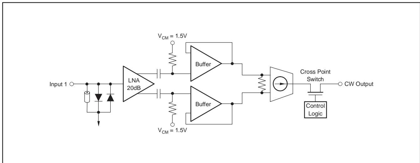
Figure 1. Basic CW Processing Block Diagram.
