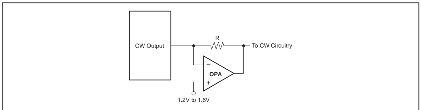
Figure 3. Operational Amplifier.
