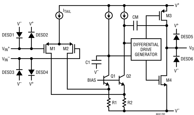
Figure 1. Simplified Schematic
