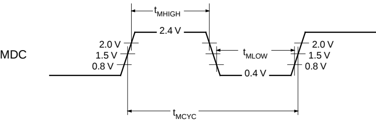
Figure 86. MDC Waveform
