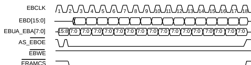
Figure 52. Typical SRAM Read Operation
