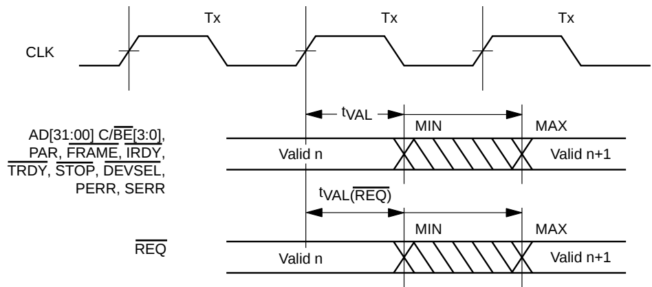
Figure 65. Output Valid Delay Timing
