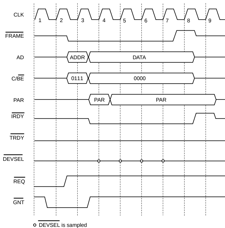
Figure 21. Master Abort
