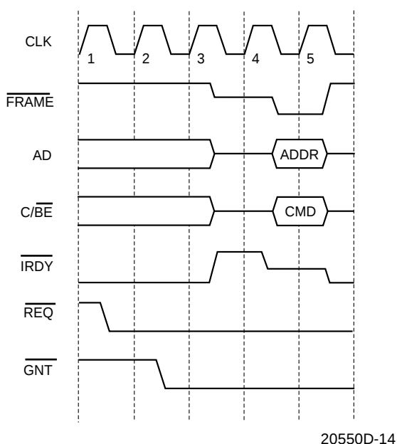
Figure 11. Bus Acquisition
