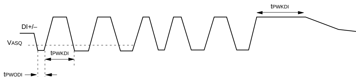
Figure 81. Receive Timing
