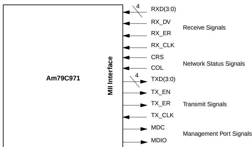
Figure 38. Media Independent Interface
