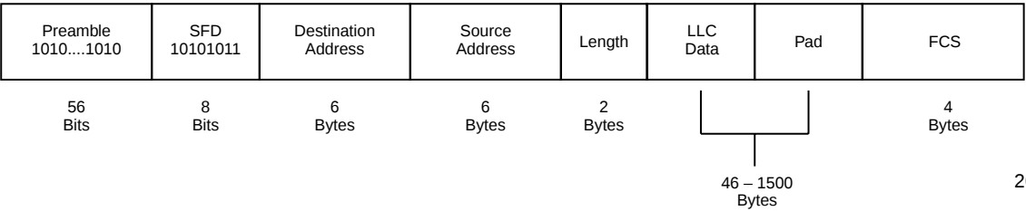
Figure 33. ISO 802-3 (IEEE/ANSI 802.3) Data Frame
