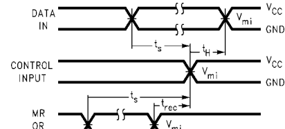
FIGURE 6. Setup Time, Hold Time and Recovery Time for Low Voltage Logic
