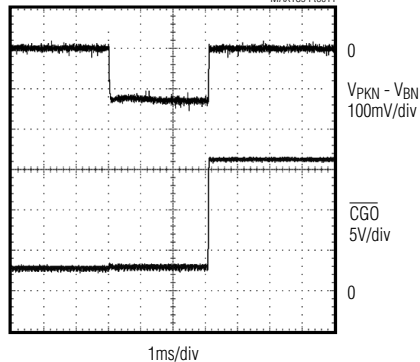
CHARGE-CURRENT FAULT TIMING
