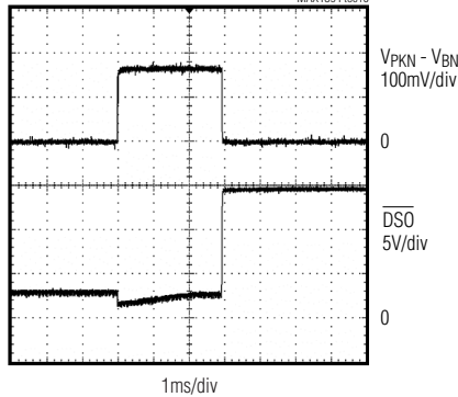
DISCHARGE-CURRENT FAULT TIMING
