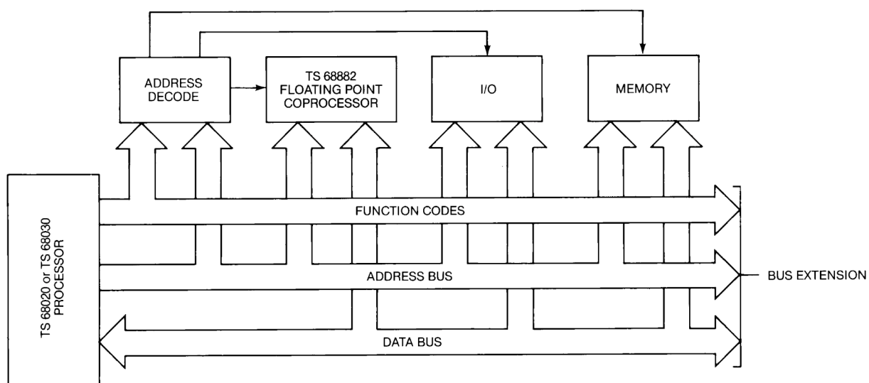
Figure 16. Typical Co-processor Configuration
