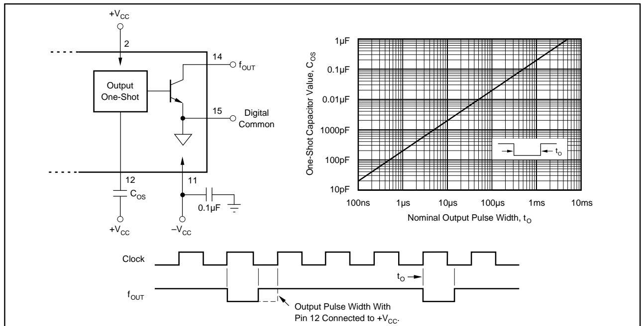
FIGURE 4. Circuit and Timing Diagram for Shortened Output Pulses.
