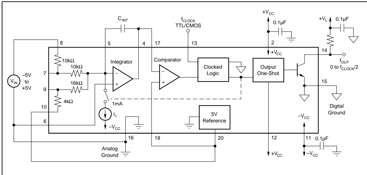
FIGURE 2. Offset for Bipolar Input Voltages.
