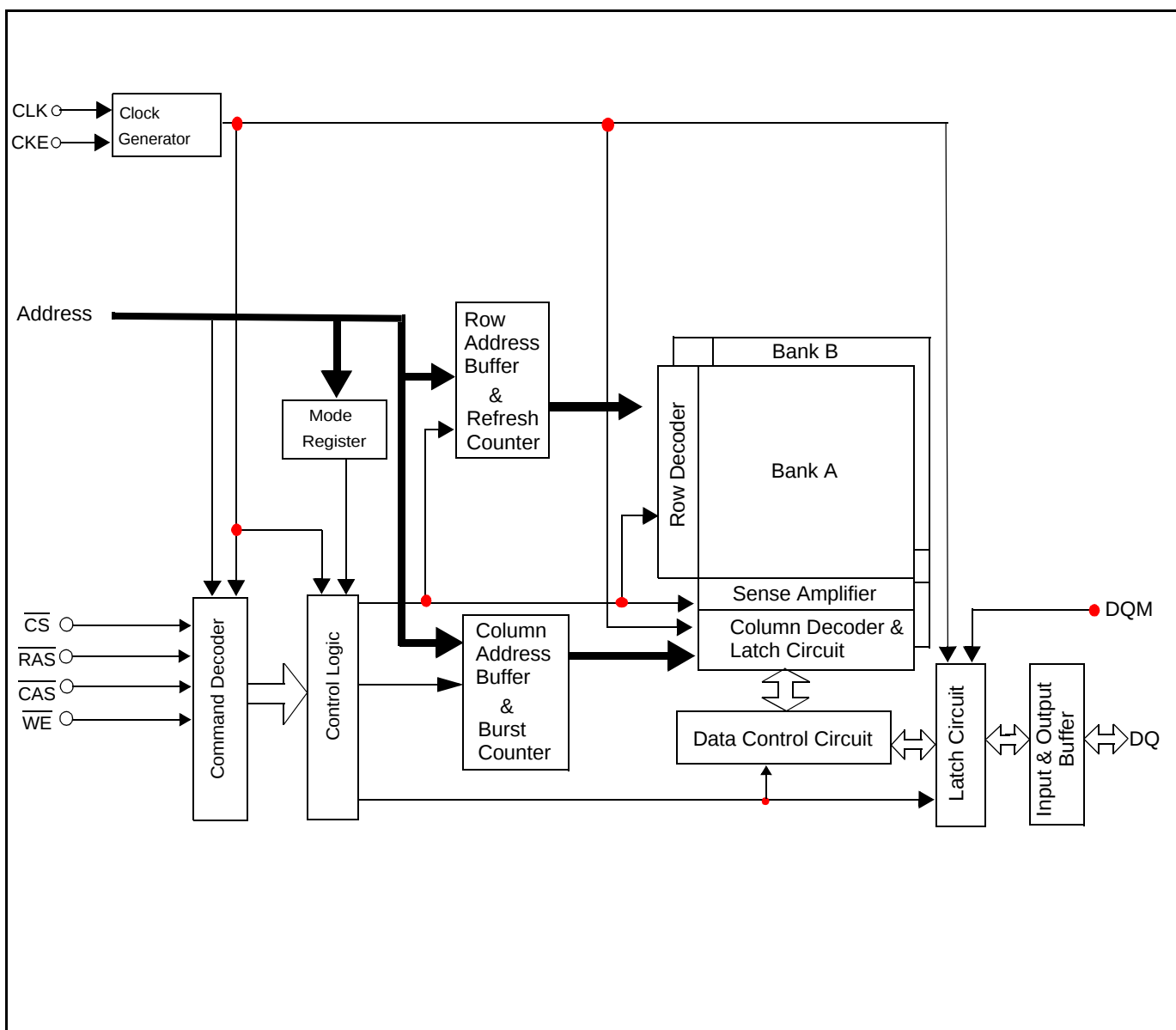
Block Diagram
