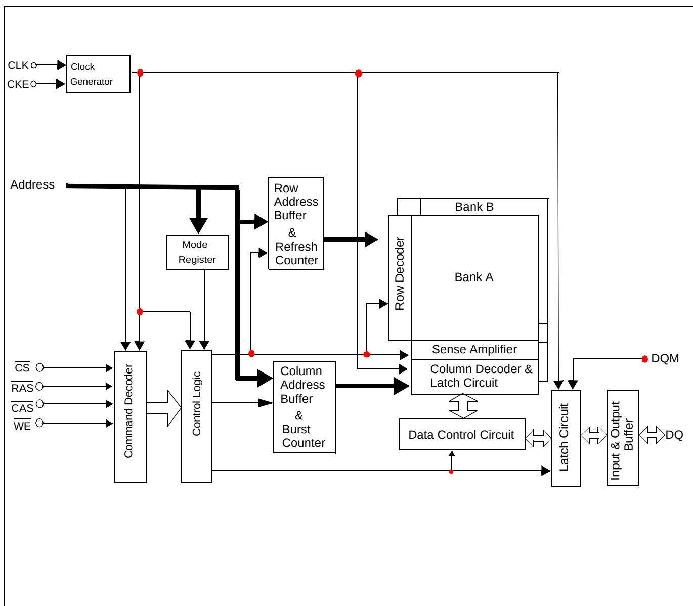
Block Diagram
