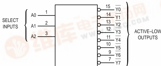
LOGIC DIAGRAM
