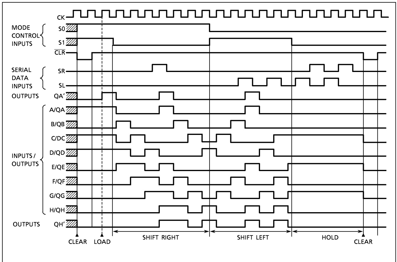
TIMING CHART
