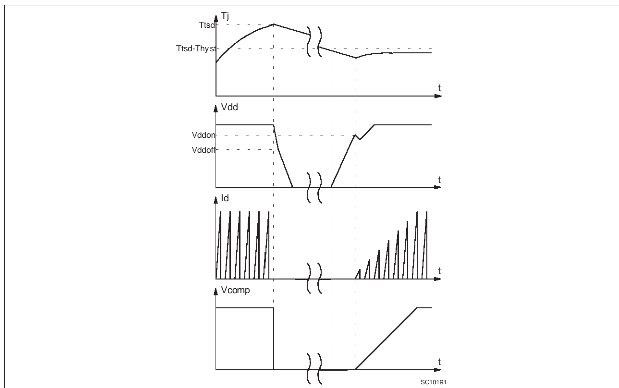
Figure 8: Overtemperature Protection
