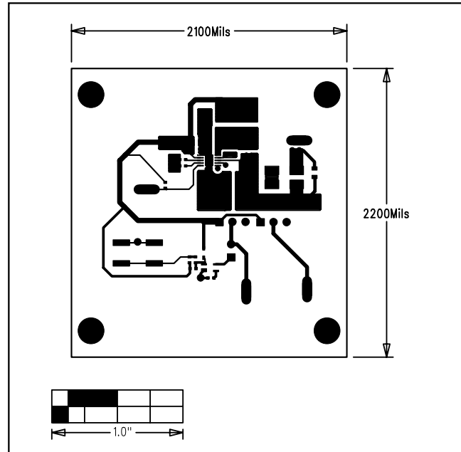
Figure 3. MAX1583 EV Kit PC Board Layout—Component Side
