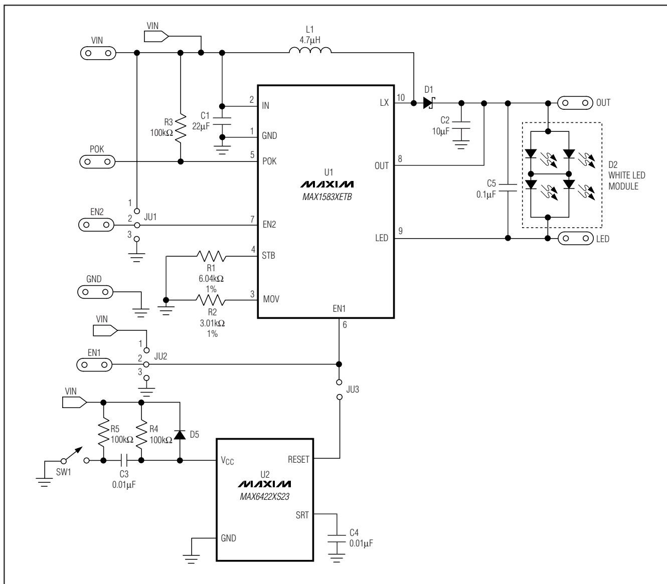
Figure 1. MAX1583 EV Kit Schematic
