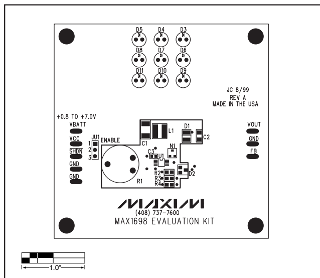
Figure 2. MAX1698 EV Kit Component Placement Guide—Component Side
