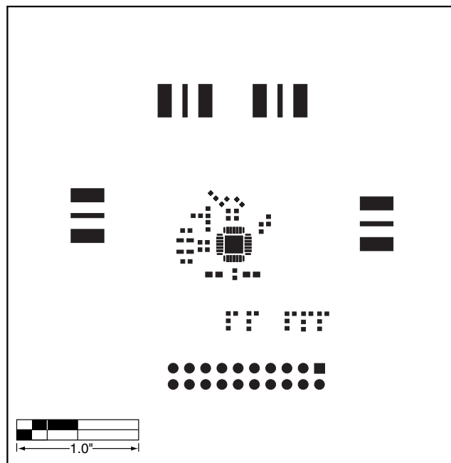
Figure 14. MAX2010 EV Kit PC Board Layout—Top Soldermask
