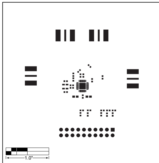
Figure 6. MAX2009 EV Kit PC Board Layout—Top Soldermask
