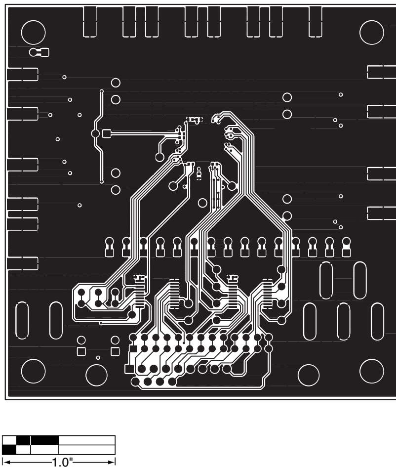
Figure 6. MAX2825/MAX2826/MAX2827 EV Kit PC Board Layout—Solder Side
