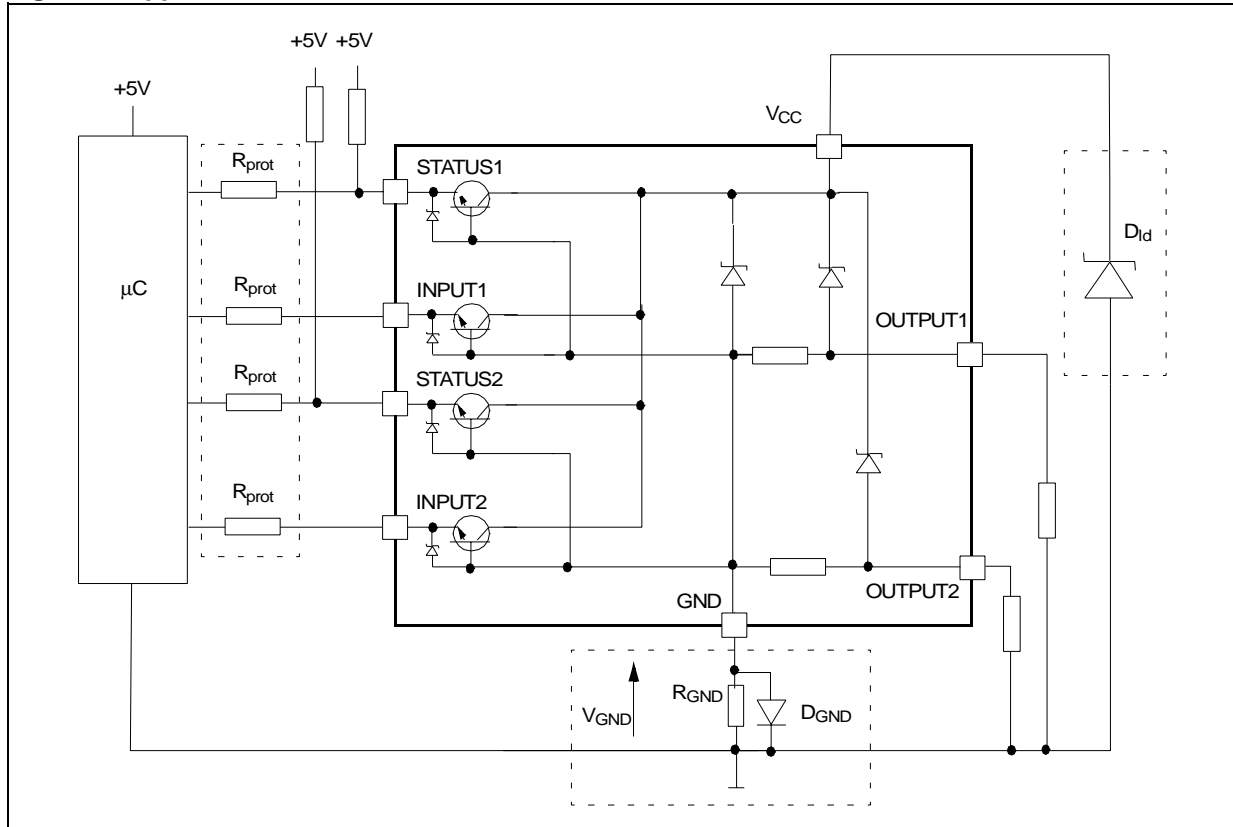
Figure 8. Application Schematic
