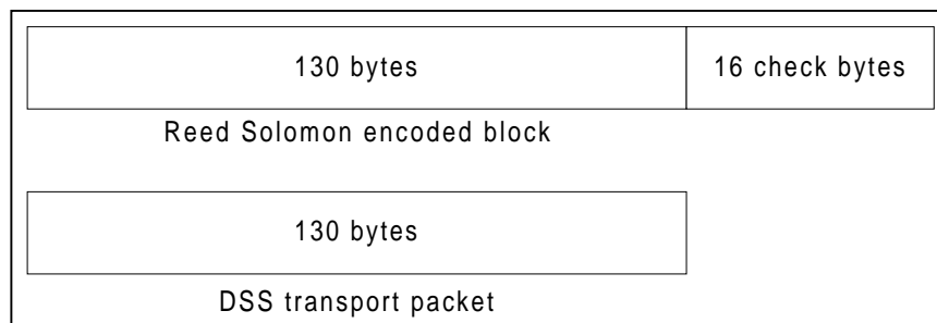
Figure 8. DSS block structure.
