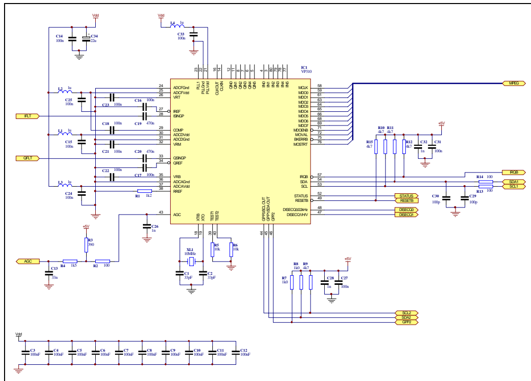
Figure 20. Application Schematic.
