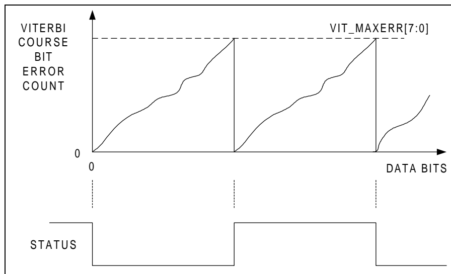
Figure 4. Viterbi error count coarse indication.
