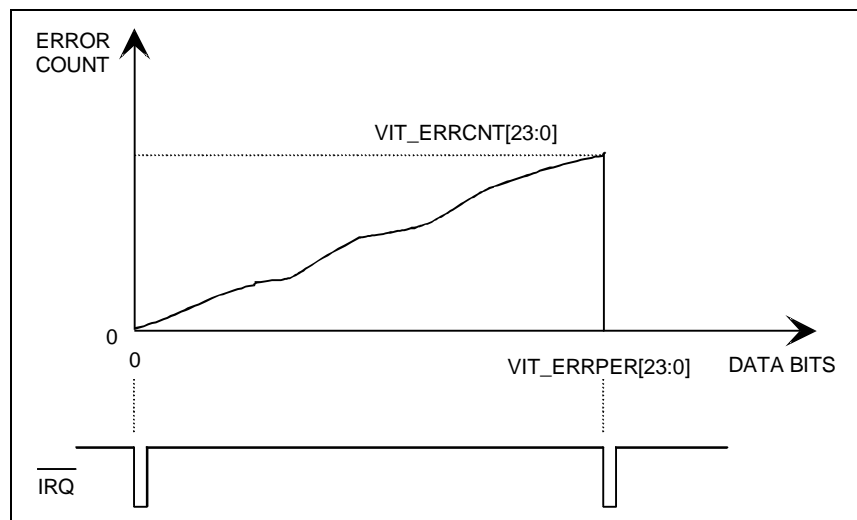
Figure 3. Viterbi error count measurement.
