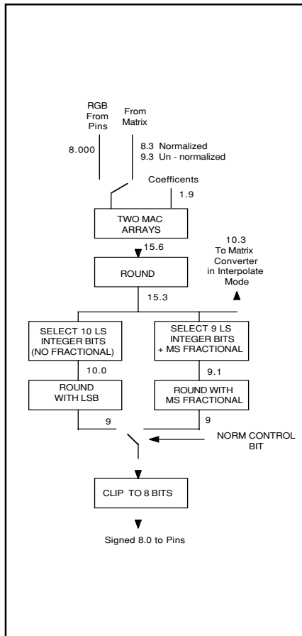
Figure 4. Bit significance
