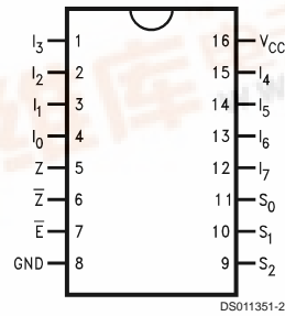
Pin Assignment SOIC JEDEC and EIAJ
