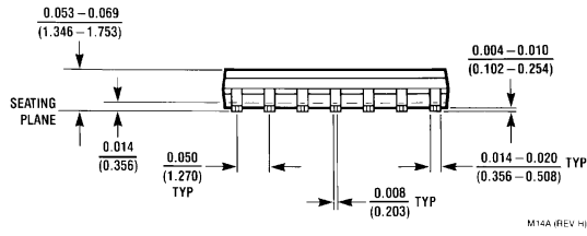
14-Lead (0.150" Wide) Molded Small Outline Integrated Circuit Package Number M14A
