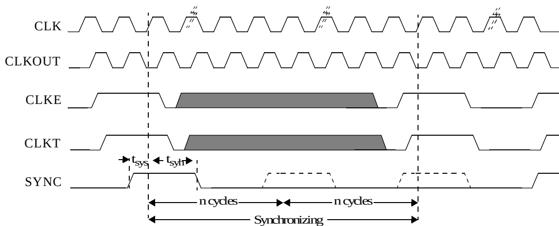
Figure 7: Synchronization Timing
