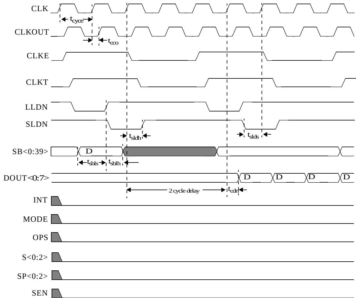
Figure 5: Multiplexer Timing (External Timing, 4:1 Mode)
