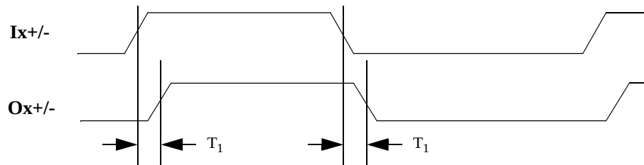
Figure 2: Timing Waveforms
