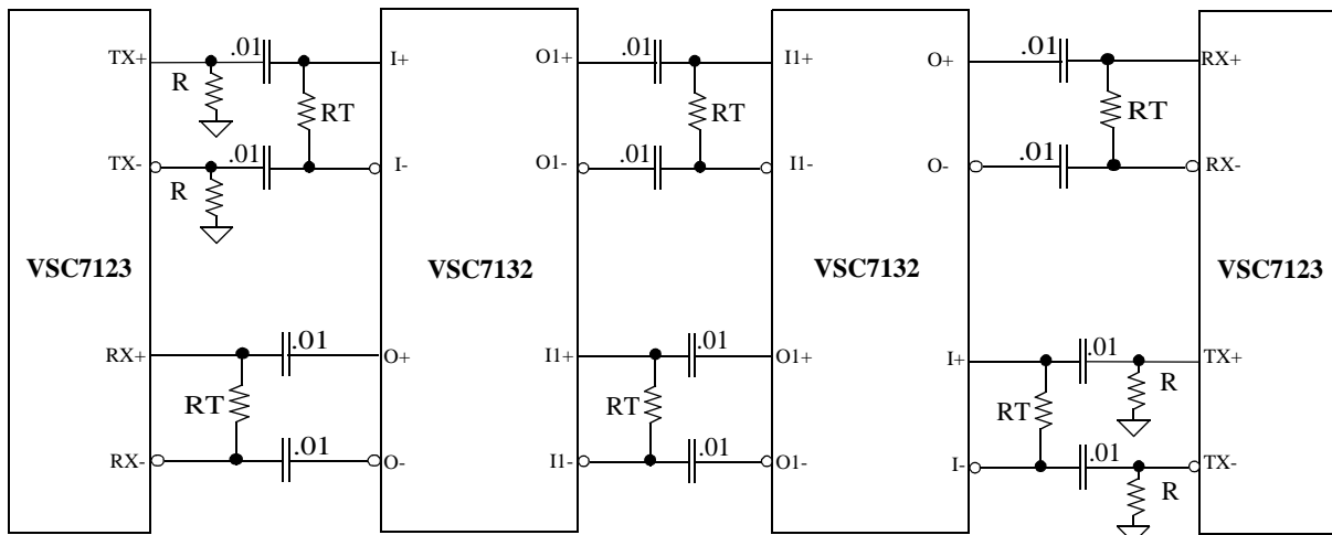
Figure 2: Application Example: VSC7123 and VSC7132 Interconnect
