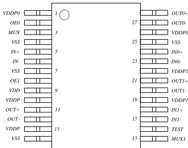
Figure 3: Pin Diagram
