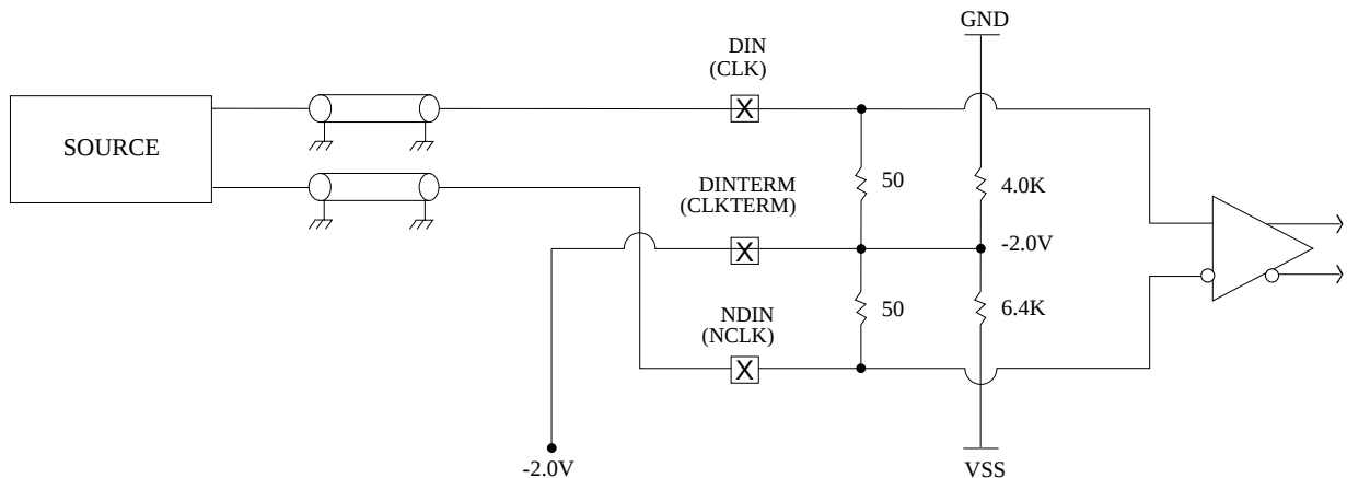
Figure 5: Differential DC-Coupled
