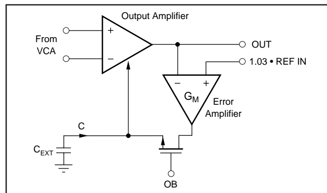
FIGURE 4. Simplified Block Diagram of Optical Black Level Auto-Zero Loop
