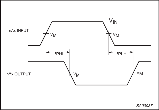
Waveform 1. Input ( n\text{Ax} ) to Output ( n\text{Yx} ) Propagation Delays
