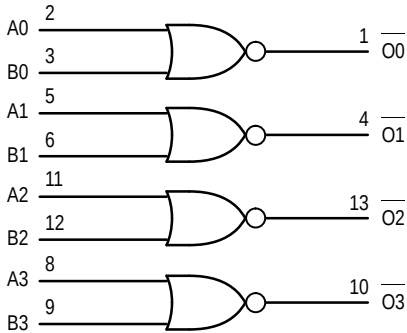
Figure 2. Logic Diagram
