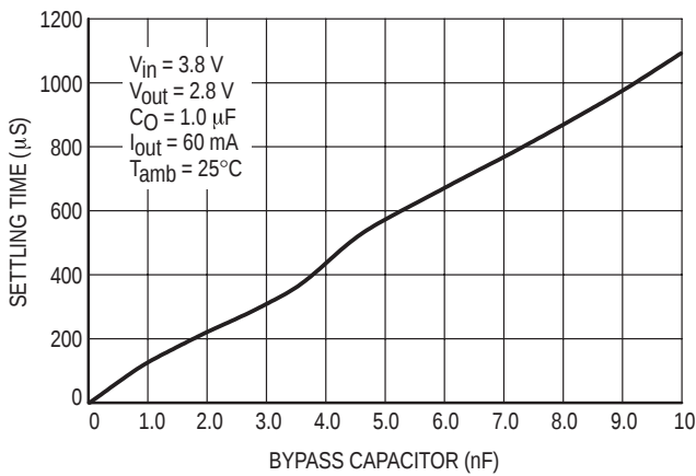
Figure 17. Output Voltage Settling Time versus Bypass Capacitor
