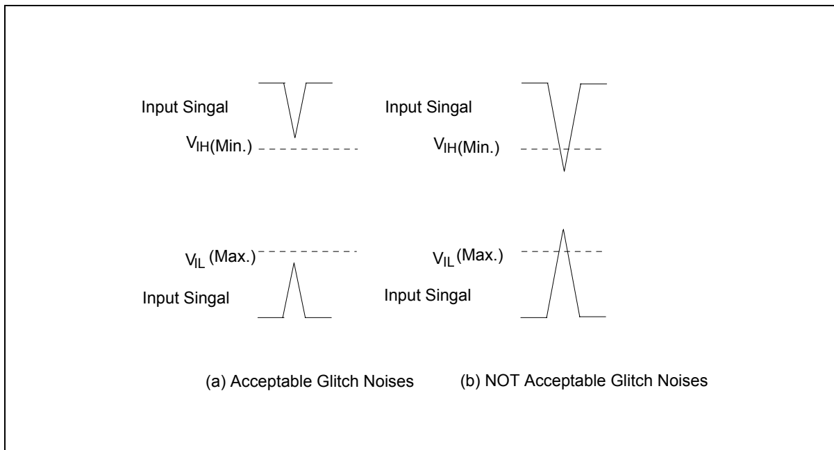
Figure 19. Waveform for Glitch Noises
