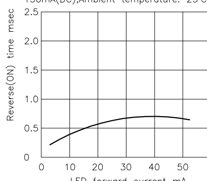
LED forward current vs. reverse(ON) time Across terminals 5,7 and 6,8 pin; Load voltage: 400V(DC); Continuous load current: 130mA(DC); Ambient temperature: 25°C
