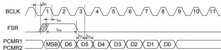
Figure 8-5b. Receive Timing
