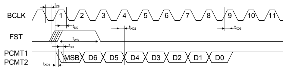
Figure 8-5a. Transmit Timing
