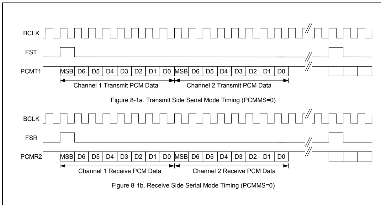
FIGURE 8.1: SERIAL MODE PCM TIMING
