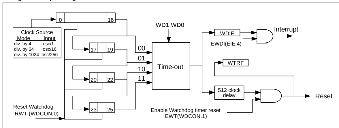
Figure 19. Watchdog Timer
