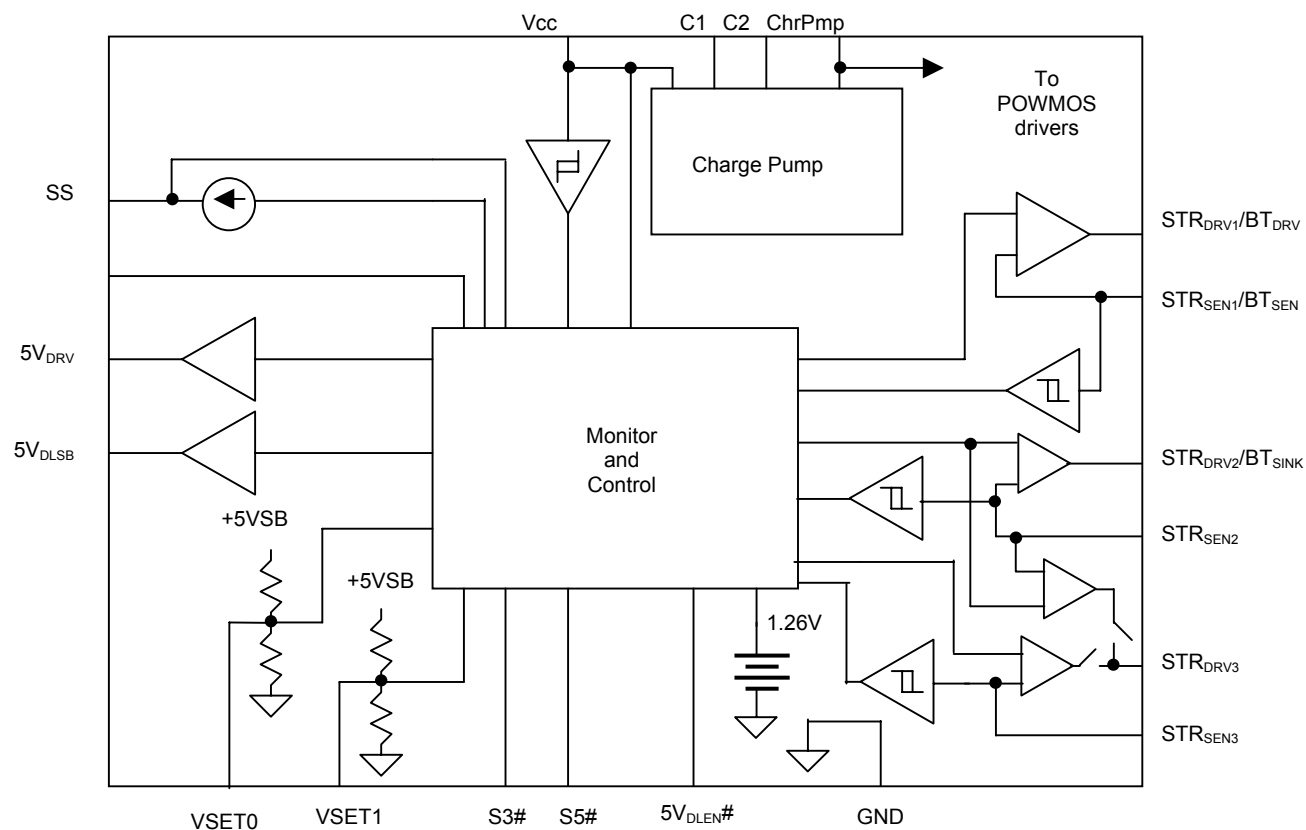
Figure 4. W83301R Internal Block Diagram
