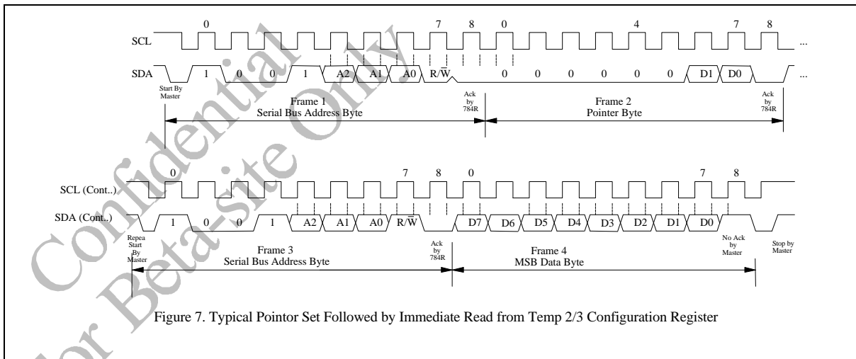
(d) Typical pointer set followed by immediate read from configuration register
