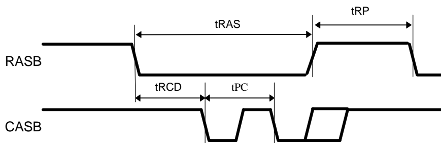
DRAM Timing
