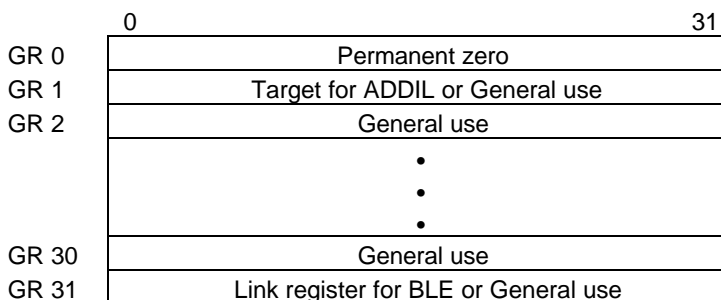
Figure 5.1 General Registers
