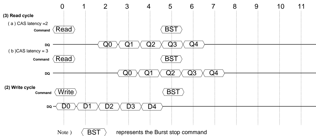
Timing chart of Burst Stop cycle ( Burst stop Command )
